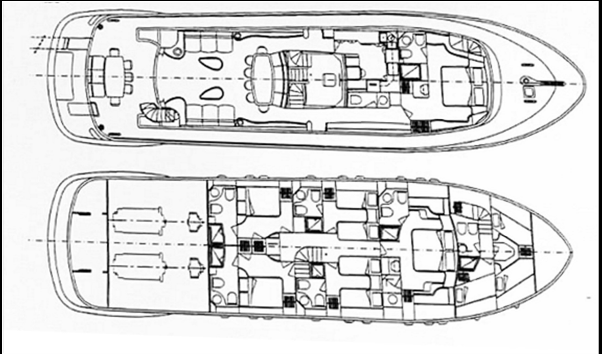
General Arrangement
